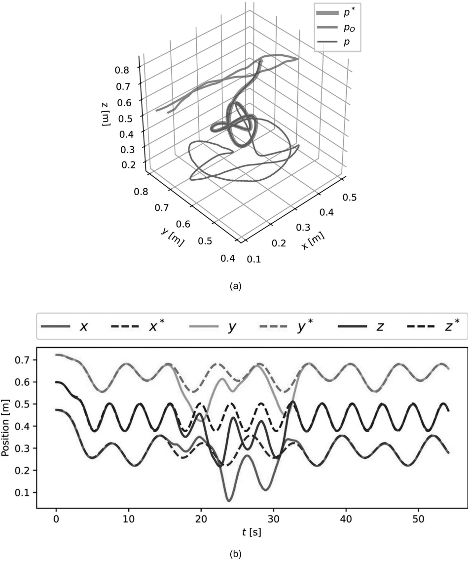
Figure 11.14 (a) As the moving obstacle with position p_O approaches the robot, the end effector position p deviates from the desired position p^* to avoid the obstacle. (b) Desired and actual xyz position of the robot end effector.
