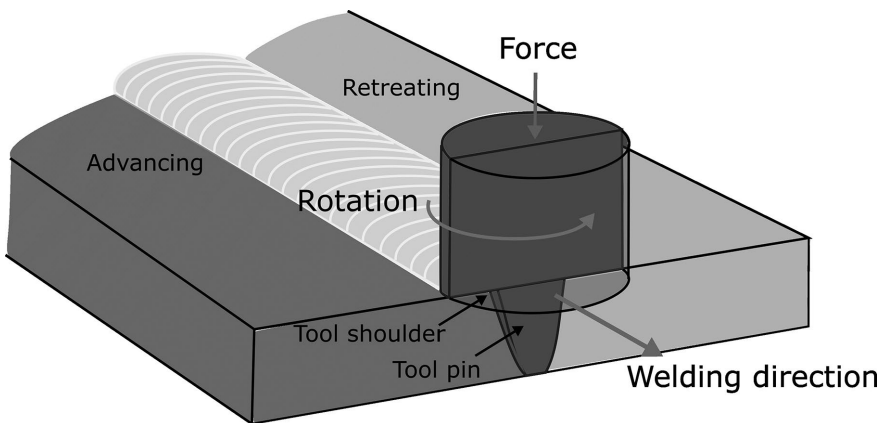
Figure 12.3 The principle of the FSW technique.
