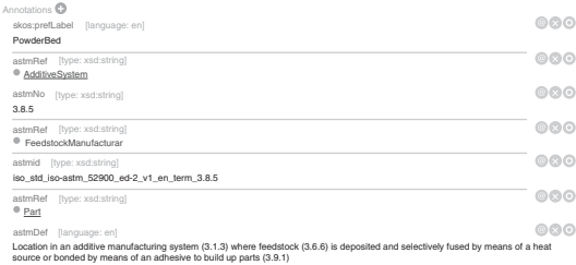
Figure 8.8 Definition and relations for the class PowderBed.
