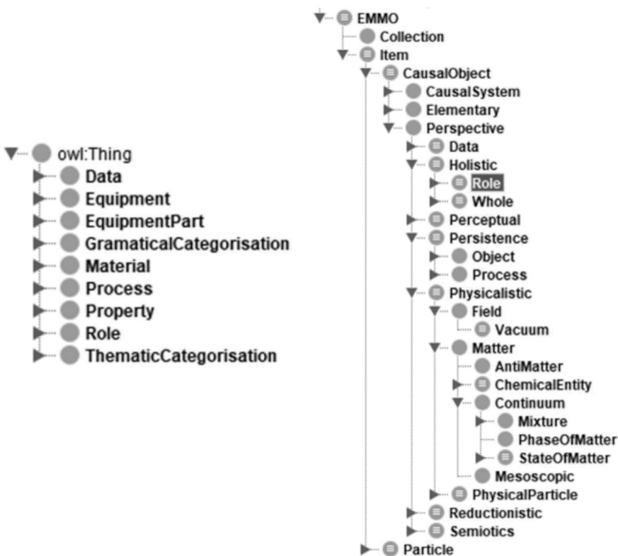
Figure 8.4 Main classes for the domain ontology for additive manufacturing (left) and the top ontology EMMO (right).
