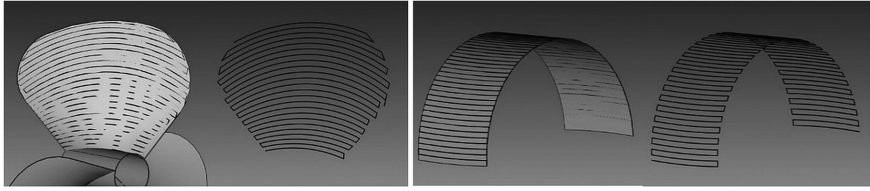
Figure 10.9 Path generated using the weighted greedy algorithm [29] (CC BY-NC-ND 4.0).
