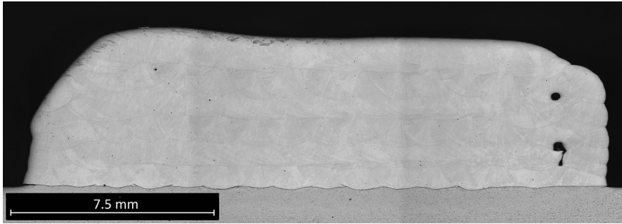
Figure 10.4 Microstructural imaging showing porosities in the finished build originating from a gap between perimeter and infill movement.
