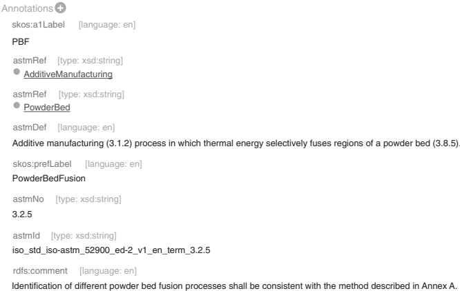
Figure 8.7 Definition and relations for the class PowderBedFusion.
