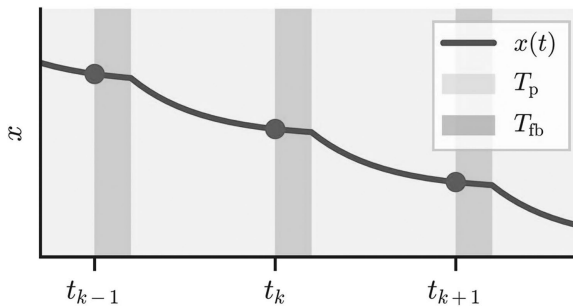
Figure 11.11 RTI loop with T_p and T_{fb} denoting the preparation phase and feedback phase, respectively. The points indicate the state sampling times.
