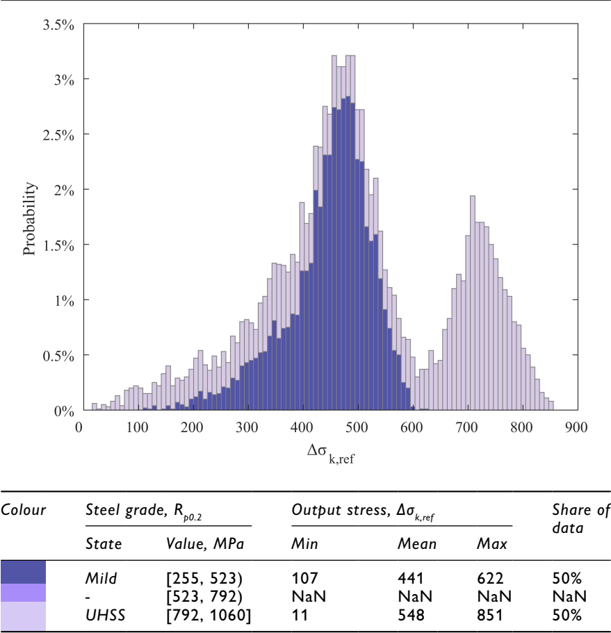
Figure 11.7 Contribution of steel grade to the variance of the output: 10% of the variance is explained by the input variable. (colour image is accessible via the link)
