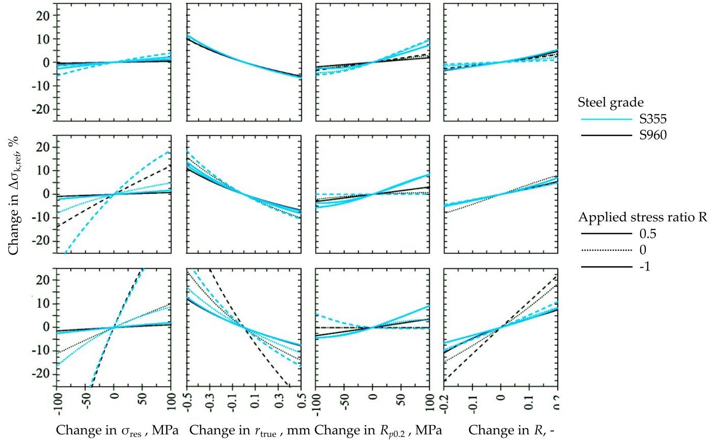
Figure 11.2 A series of one-at-a-time sensitivity analyses of 4R model output to the four inputs (in columns). The rows represent different levels of residual stress \sigma_{res} : high (upper row), negligible (middle row), and compressive (lower row). (colour image is accessible via the link)
