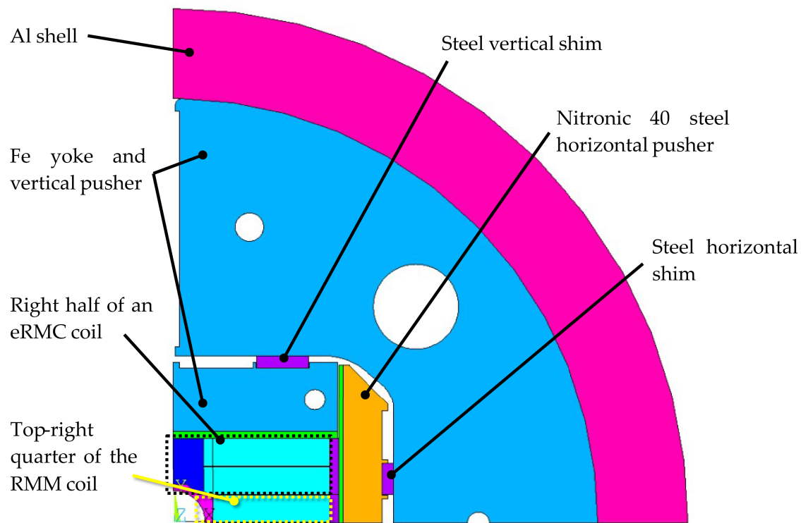
Figure 12.8 2D model of the RMM magnet, depicting a simplified geometry. (colour image is accessible via the link)
