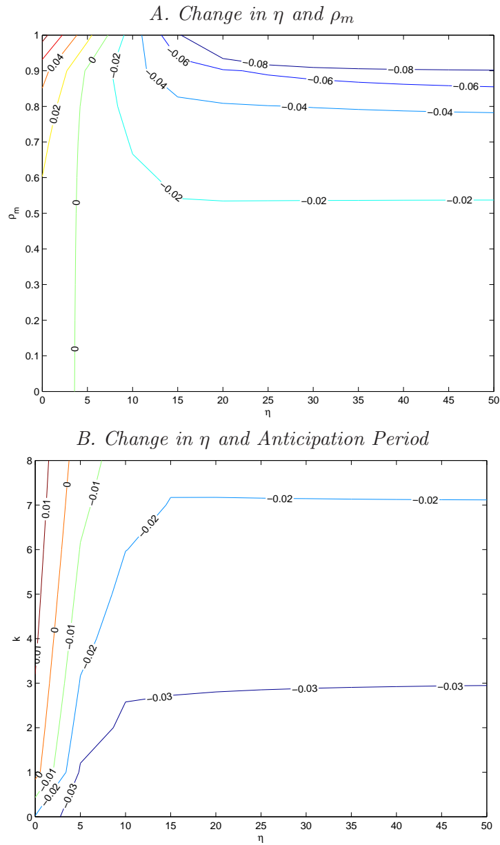
Figure 3: Maximum Response of the Output Gap to Anticipated Money Supply Shock: Sticky Price Model
