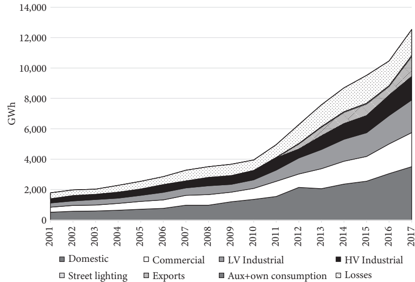
Figure 8.7 Electricity generated by end purpose
