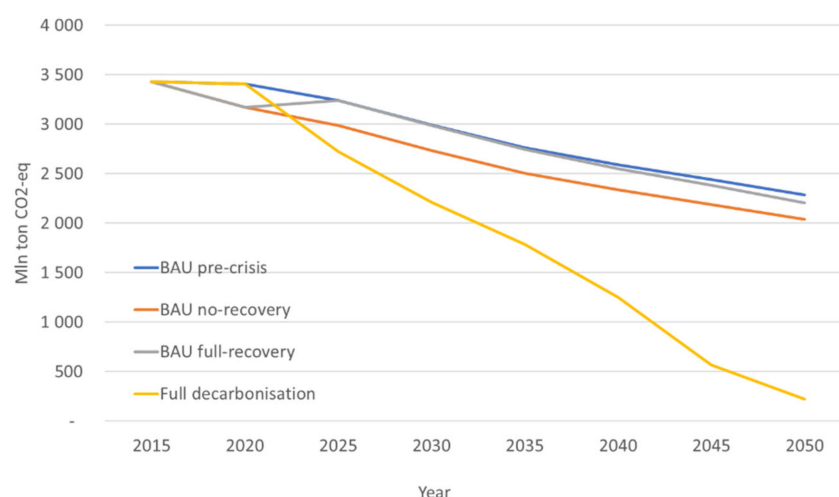
Figure 6. CO 2 emissions pattern in EU27 in reference cases (own elaboration on GDynEP results).
