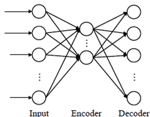
Figure 1. Autoencoder structure.
