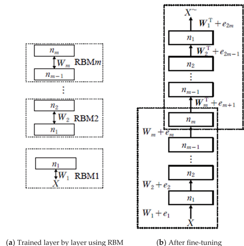
Figure 3. Proposed model based on RBM.
