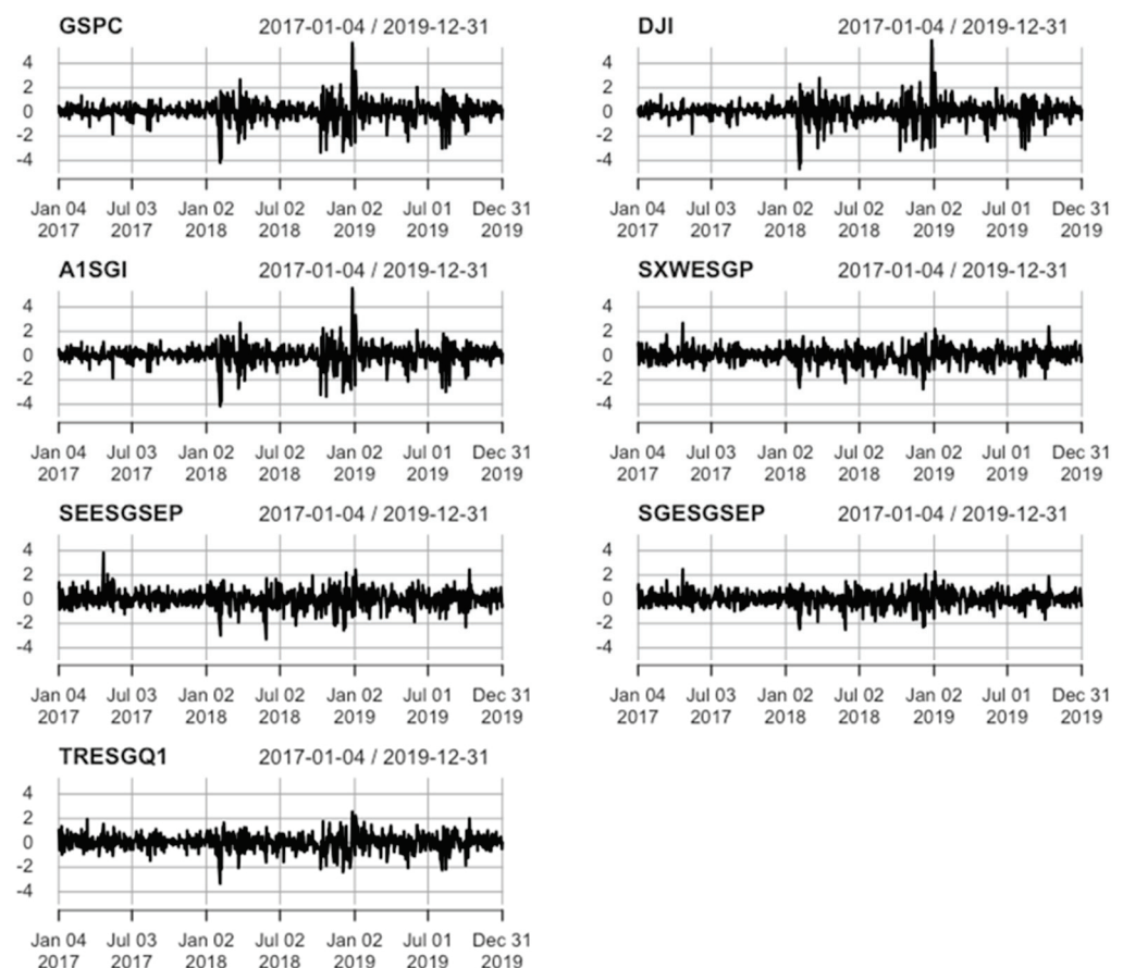
Figure 7. The rates of return, 4 January 2017–31 December 2019.
