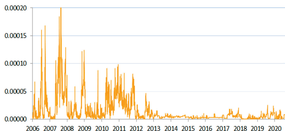
Figure 1. SIN measure for Czechia between 2006 and 2020.
