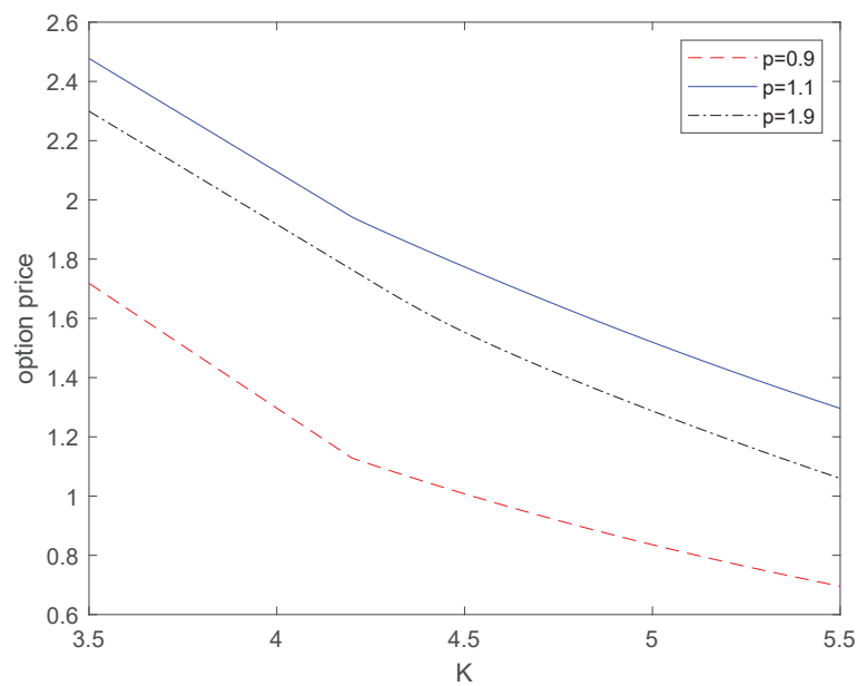
Figure 5. Price of the option with different K in [3.5, 5.5] while p is constant.
