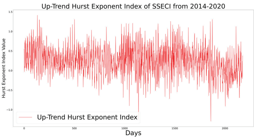
Figure 5. The graph of up-trend Hurst exponent index of SSECI.
