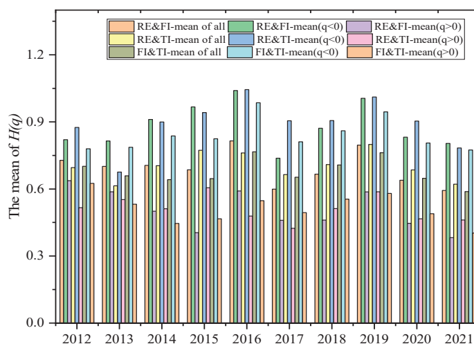
Figure 5. Tim-evarying memory analysis of H(q) mean among TI, FI, and RE.
