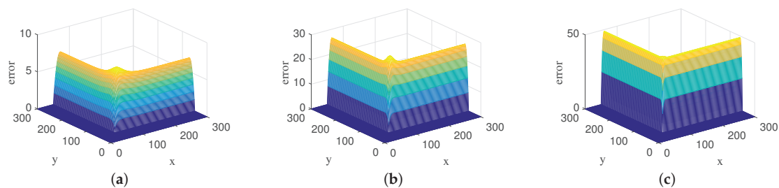
Figure 8. (a) denotes |kv - v| for different x, y when H_x = H_y = 0.3 , (b) denotes |kv - v| for different x, y when H_x = H_y = 0.5 and (c) denotes |kv - v| for different x, y when H_x = H_y = 0.7 .
