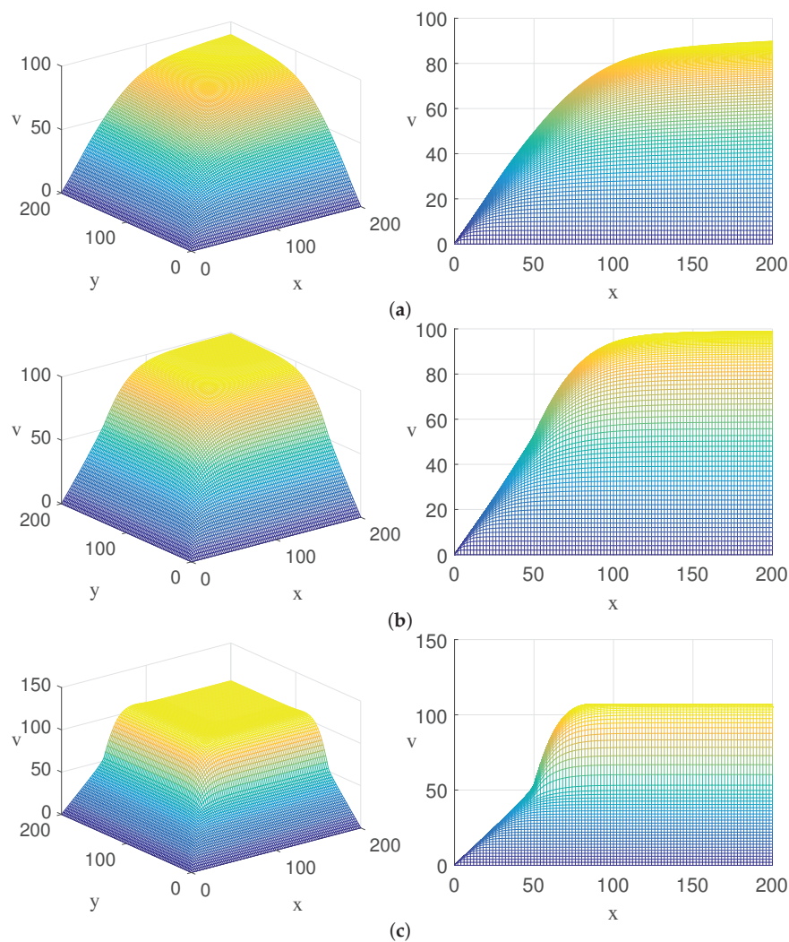
Figure 10. (a) denotes v for different x, y when H_x = H_y = H_z = 0.3 and z = 100 , (b) denotes v for different x, y when H_x = H_y = H_z = 0.5 and z = 100 and (c) denotes v for different x, y when H_x = H_y = H_z = 0.7 and z = 100 .
