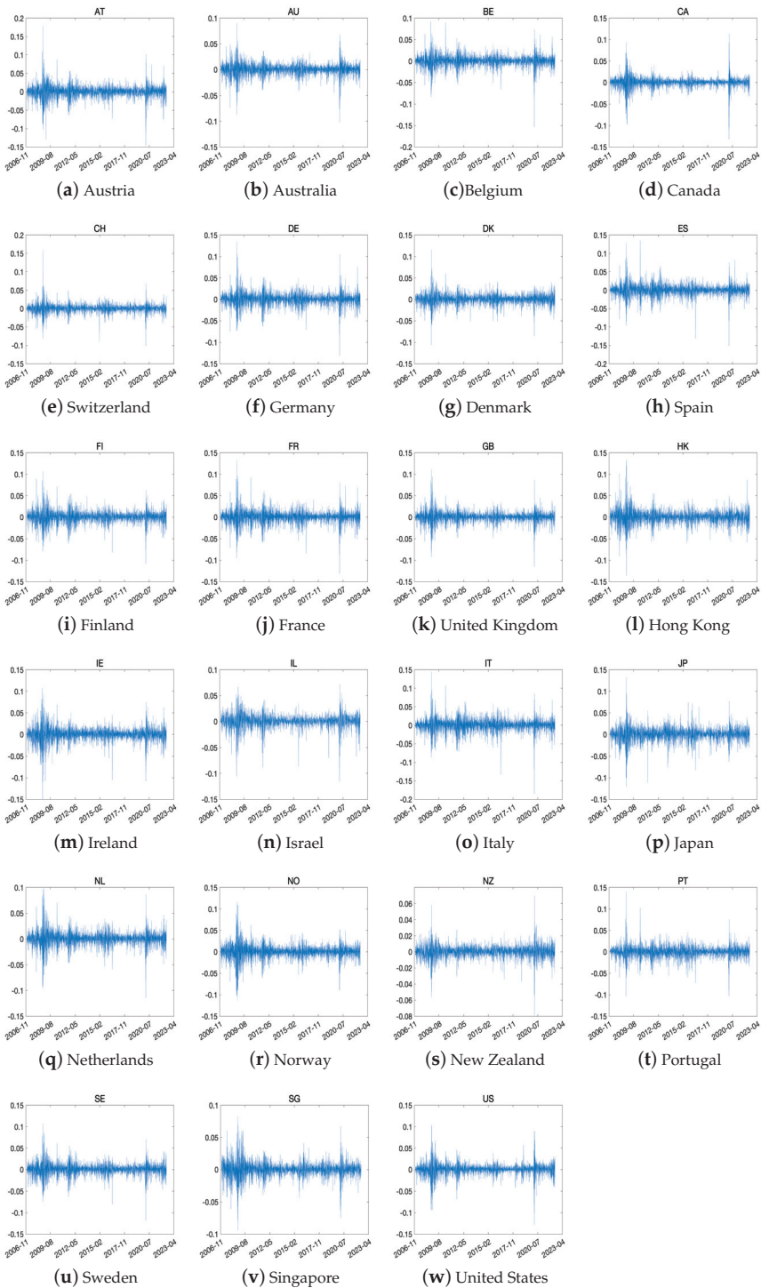
Figure 1. The log return time series for all the indices in developed countries.
