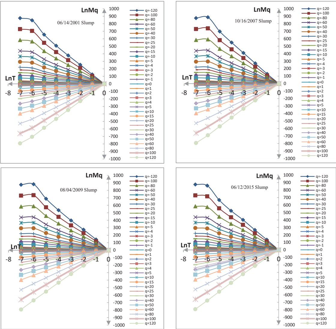
Figure 1. Curves of \ln M_q(T) vs. \ln(T) with different values of q .
