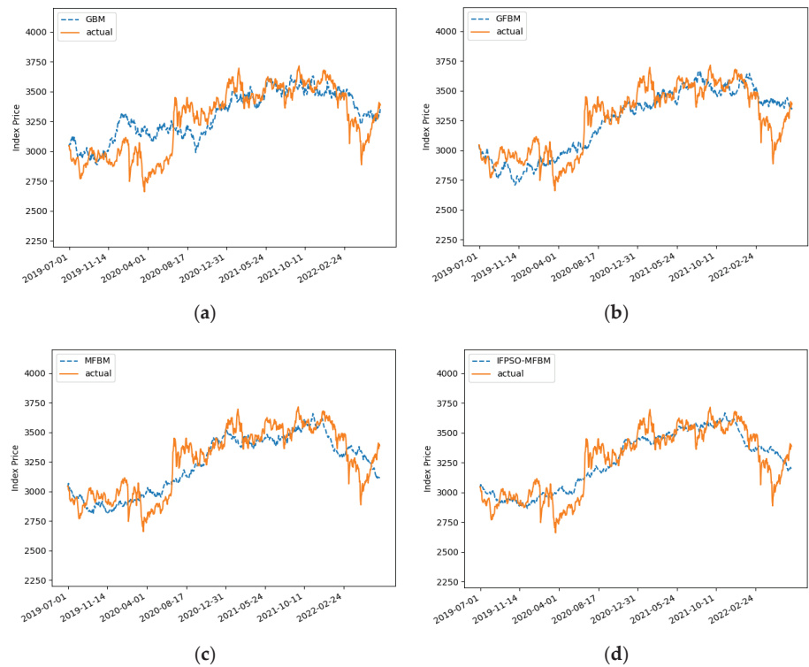
Figure 4. Comparison of the true and predicted values of SSE under the four models. (a) GBM, (b) GFBM, (c) MFBM, (d) IFPSO-MFBM.
