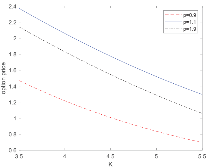
Figure 2. The price of the option with different K in [3.5, 5.5] while p is constant.
