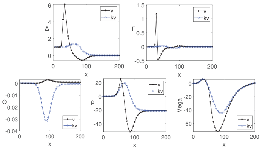
Figure 14. H_x = H_y = H_z = 0.5 , figures represent in turn are Delta, Gamma, Theta, Rho and Vega. The blue curve stands for option price with knock-in-barrier while the black curve represents option price without knock-in-barrier. For interpretation of the references to color in the figure, the reader is referred to the web version of the article.
