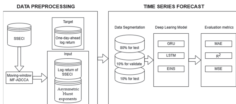
Figure 7. Flowchart of time series prediction implementation.
