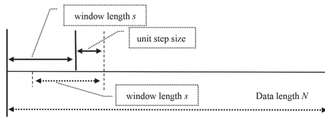
Figure 1. Details of sliding-window segmentation.
