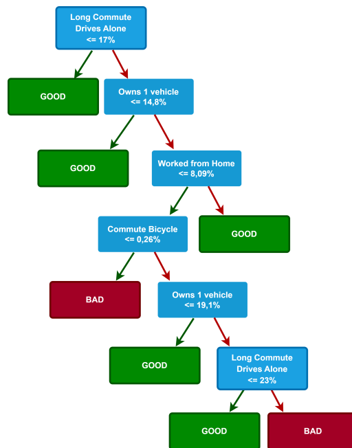
Figure 6: From WEKA: Output - Tree
