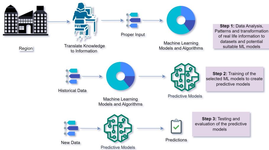
Figure 8: Methodology Overview
