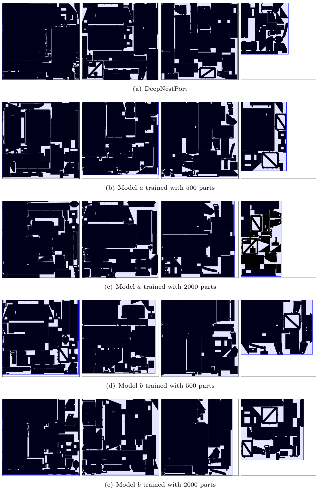
Fig. 11 Nesting layouts for experiments in section “ Comparison of GRG with open-source Nesting software ” on Test Split 1 (regular shapes)
