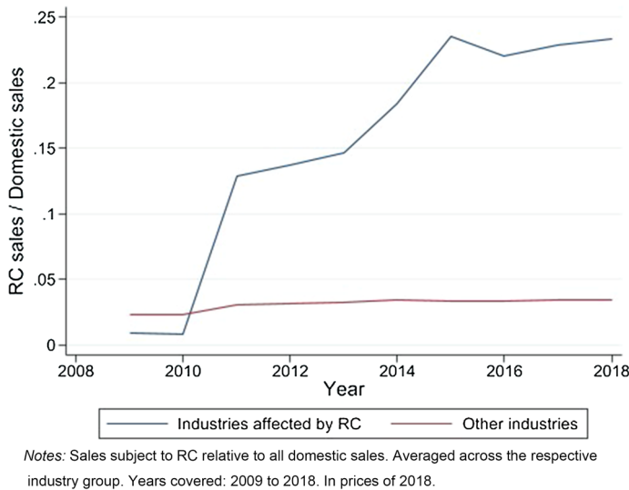
Fig. 2 Fraction of Sales Subject to RC: Non-/Affected Industries
