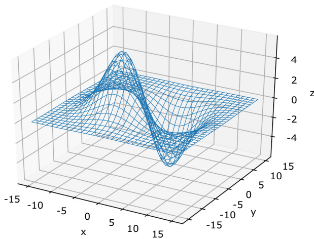
Fig. 5 Total derivative of the two dimensional Gauss function given in Eq. 3. This kernel offers versatile filter settings and reliable edge detection
