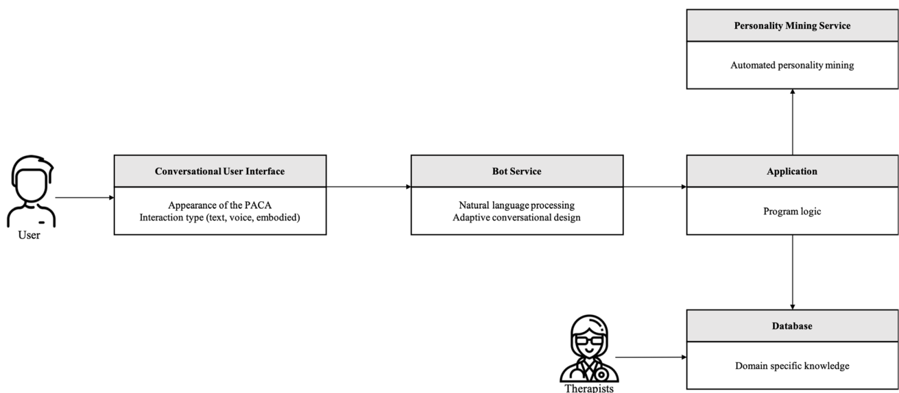
Fig. 3 Expository instantiation
