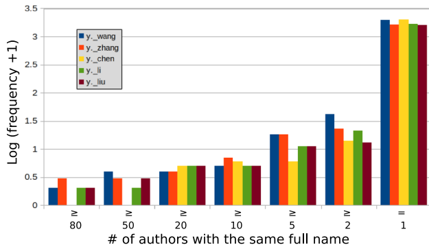
Fig. 3 The log frequency of authors sharing the same full name for the top five sub-collections (colour figure online)
