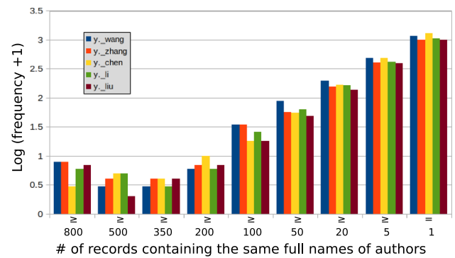
Fig. 4 The log frequency of records with the same full name of the target author for the top five sub-collections (colour figure online)
