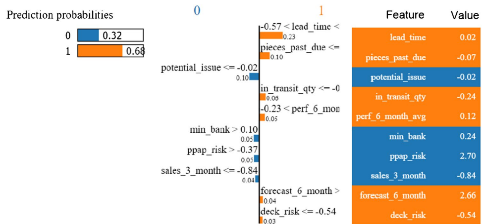
Fig. 7 Local explanations of an individual prediction using LIME
