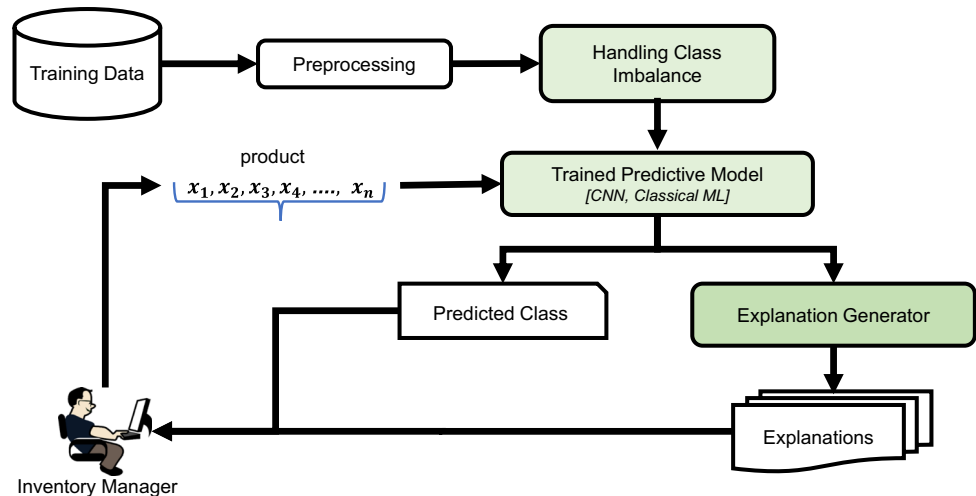
Fig. 1 Proposed explainable backorder prediction approach
