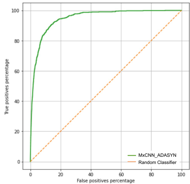
Fig. 4 Performance of convolutional neural network based predictive model in terms of Receiver Operating Characteristic curve (ROC curve). The X-axis and Y-axis indicate the false positive and true positive percentage, respectively
