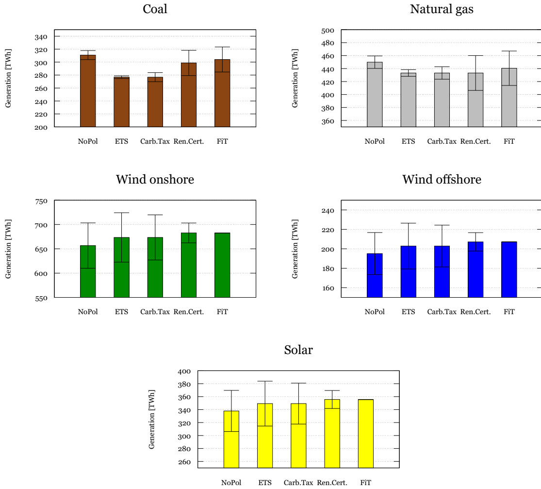
Figure 1: Mean generation per variable technology.
