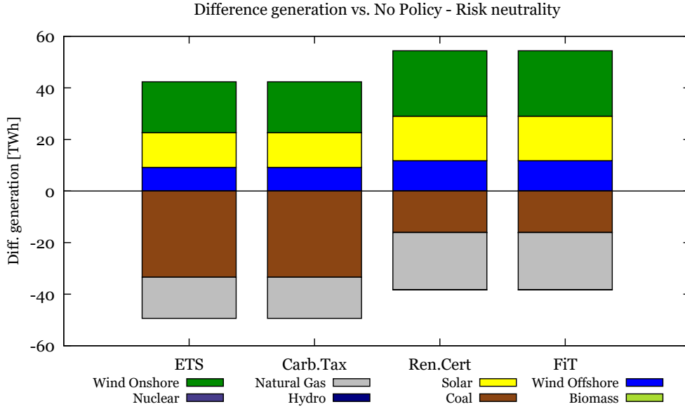
Difference between policy scenario and No policy in TWh of electricity generation per technology under risk neutrality ( \gamma = 0 ).
