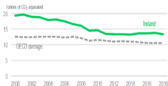
Figure 4. Greenhouse Gas emissions per capita
