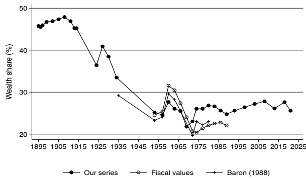
(a) Using fiscal values as in Baron (1988)
