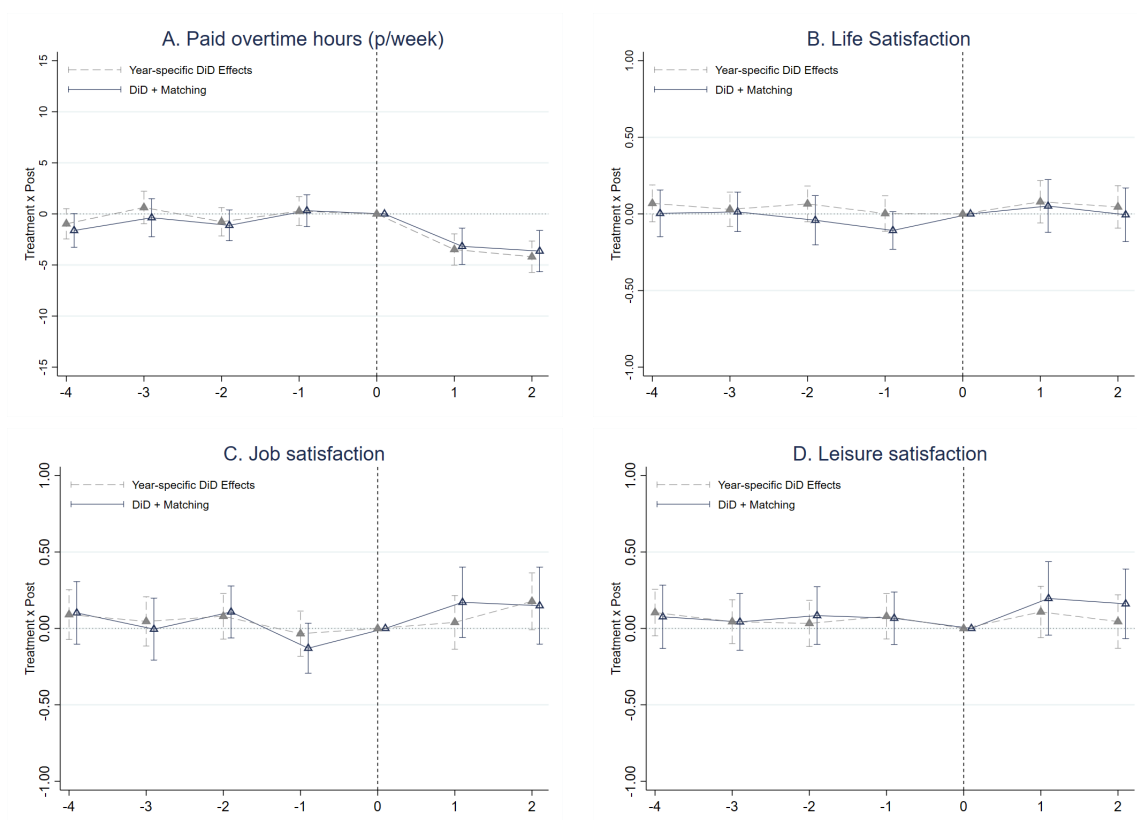
Figure 6: Event-Study Analysis: Self-Reported Overtime and Subjective Well-Being
