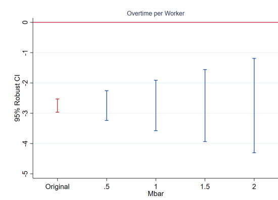
Figure A2: Honest Pre-Trends (Rambachan and Roth, 2023)
