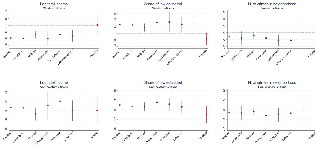
Figure 6: Robustness tests
