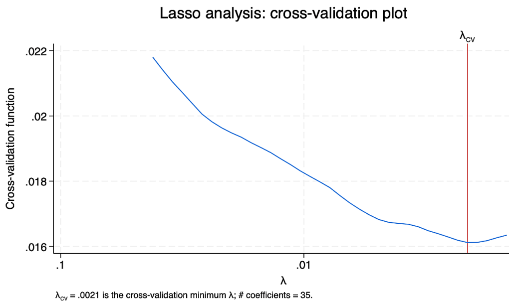
Figure 4: Lasso Analysis: Cross-Validation Plot
