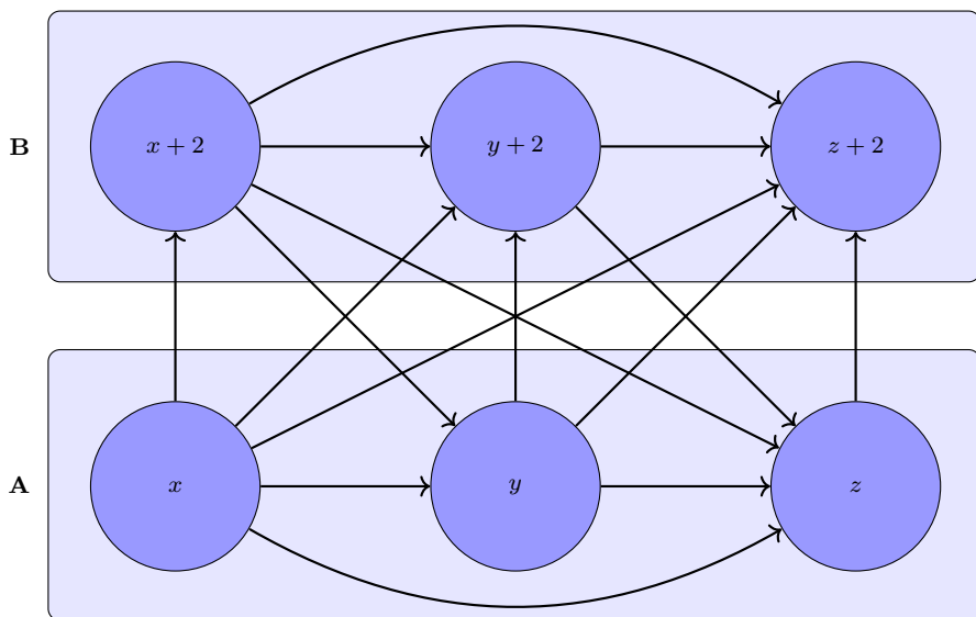
Fig. 4 Graphical representation of a preordered space, defined in Proposition 3, which has multi-utilities with cardinality c and no strict monotone. In particular, we show A := [0, 1] , B := [2, 3] and how x, y, z \in A , x < y < z , are related to x + 2, y + 2, z + 2 \in B . Notice, an arrow from an element w to an element t represents w < t
