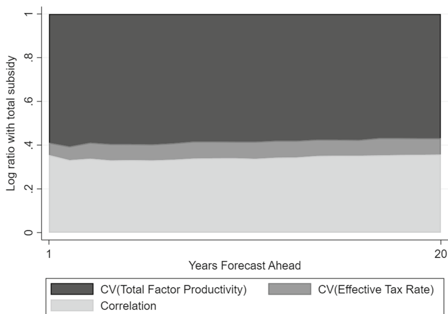
Fig. 1 Decomposition of the effects resulting in the estimated T over a 20-year window, as in Eq. 9
