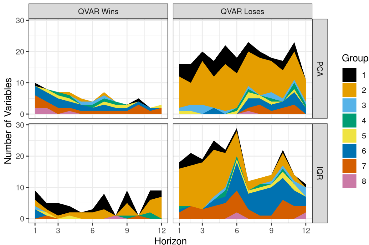
FIGURE 8. QVAR and QFAVAR Recesssion Comparison (tail-weighted CRPS)
