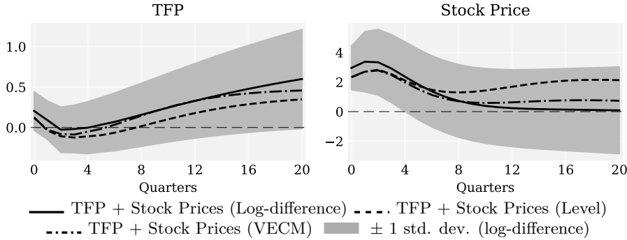
Figure 14: IRF of TFP and the Stock Price Index
