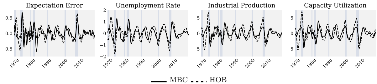
Figure 8: MBC vs HOB: Conditional History
