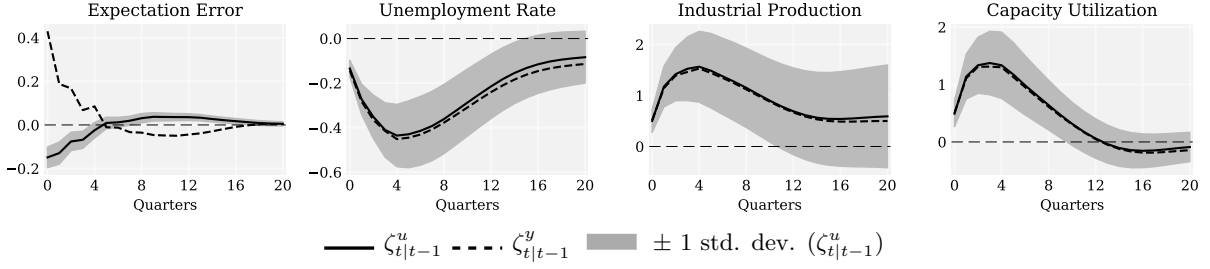
Figure 20: Impulse Response to a HOB Shock: Output vs Unemployment Expectation Error
