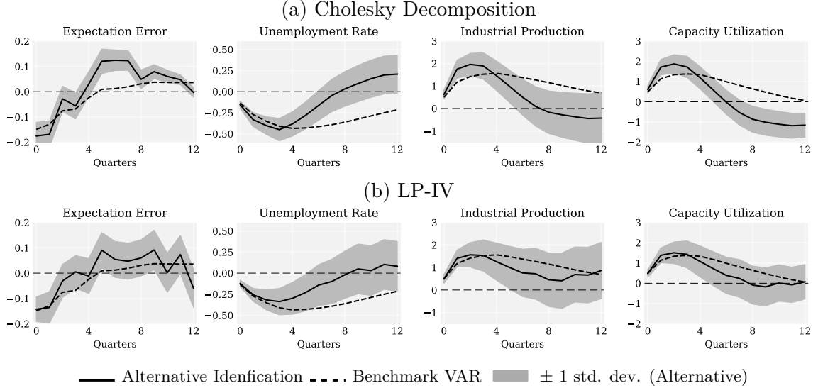
Figure 22: Alternative Identification Strategies: IRFs
