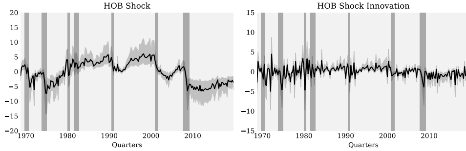
Figure 1: A Variety of Models
