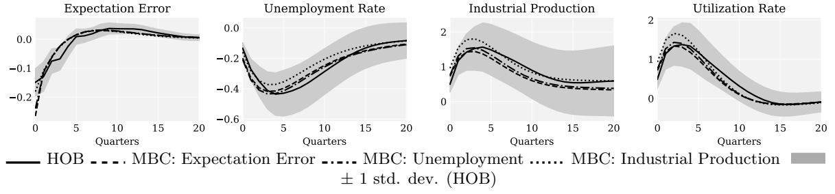
Figure 7: Extended VAR on MBC component: IRFs
