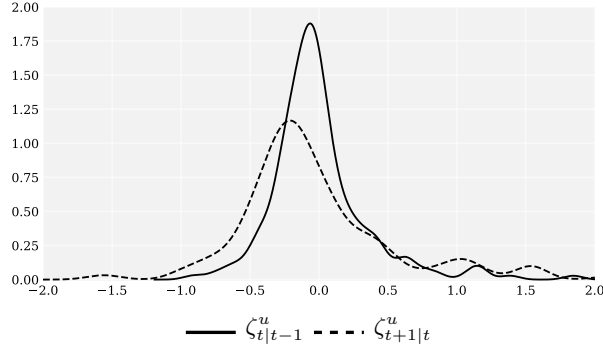
Figure 18: Distribution of Expectation Errors: Timing
