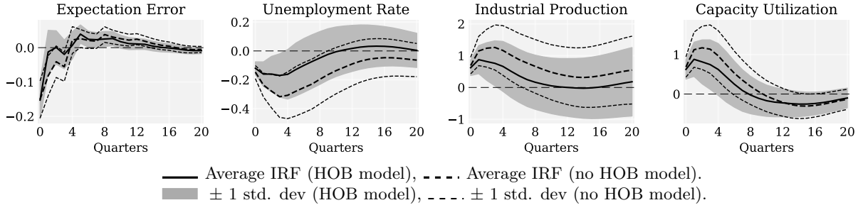
Figure F.2: Impulse Response to a Transitory Investment Shock
