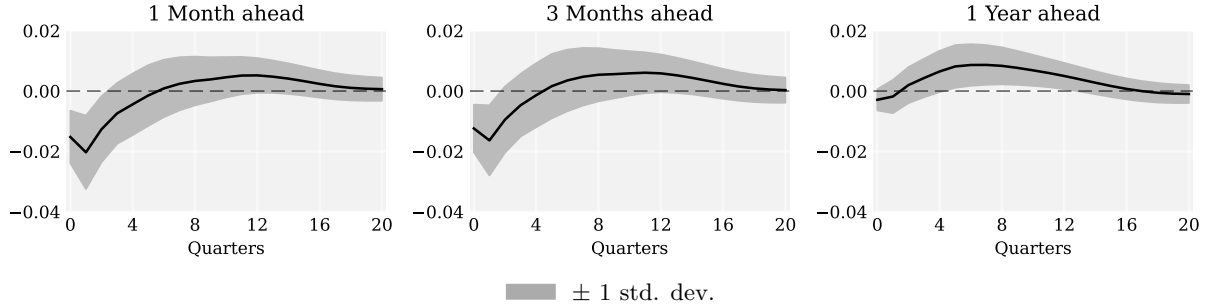
Figure 9: IRF of Uncertainty Measures
