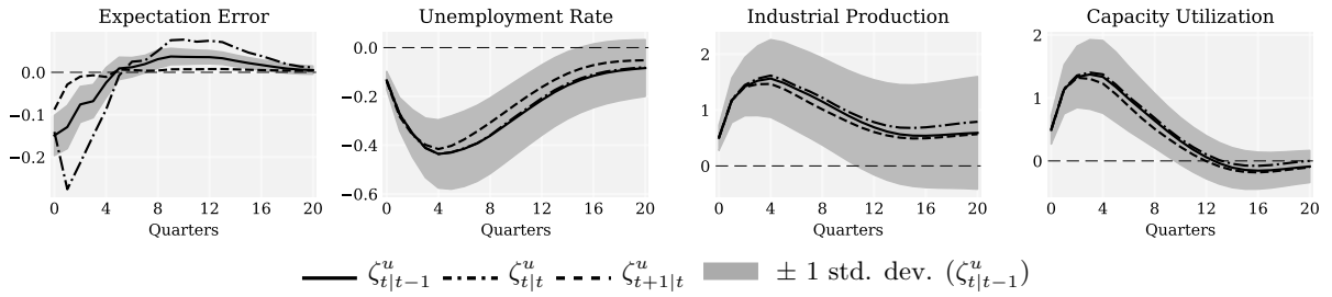
Figure 19: Impulse Response to a HOB Shock: Varying the timing of Expectations
