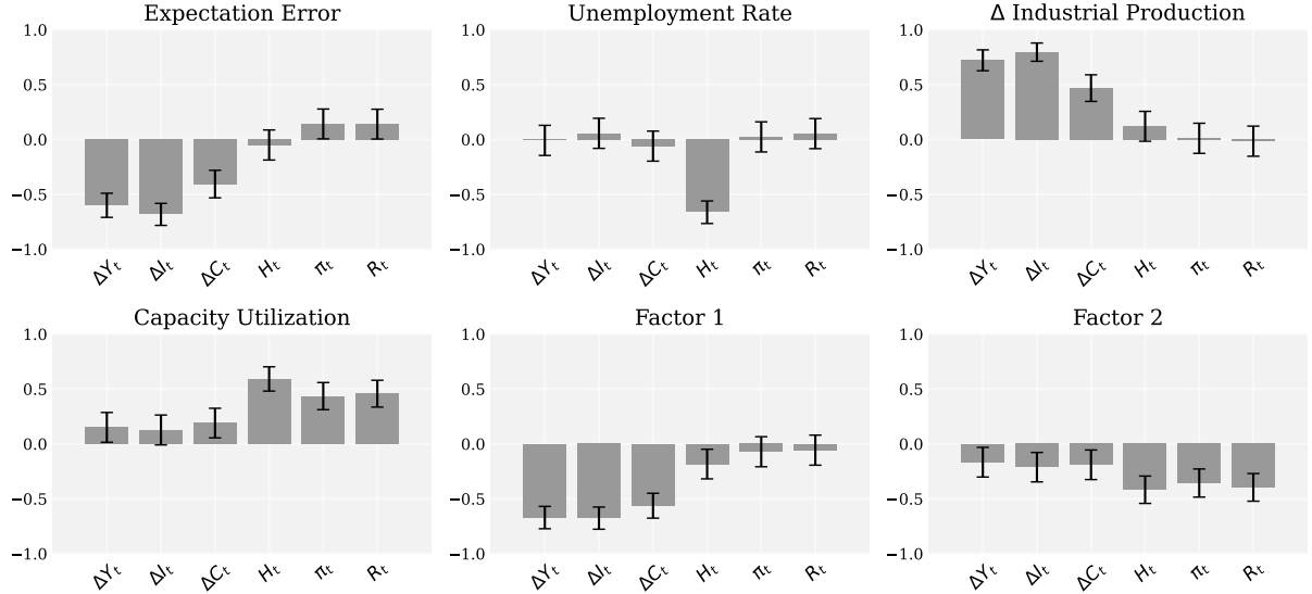
Figure A.1: Correlation Analysis
