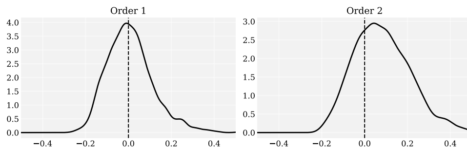
Figure B.1: Serial Correlation of the Instrument across Models
