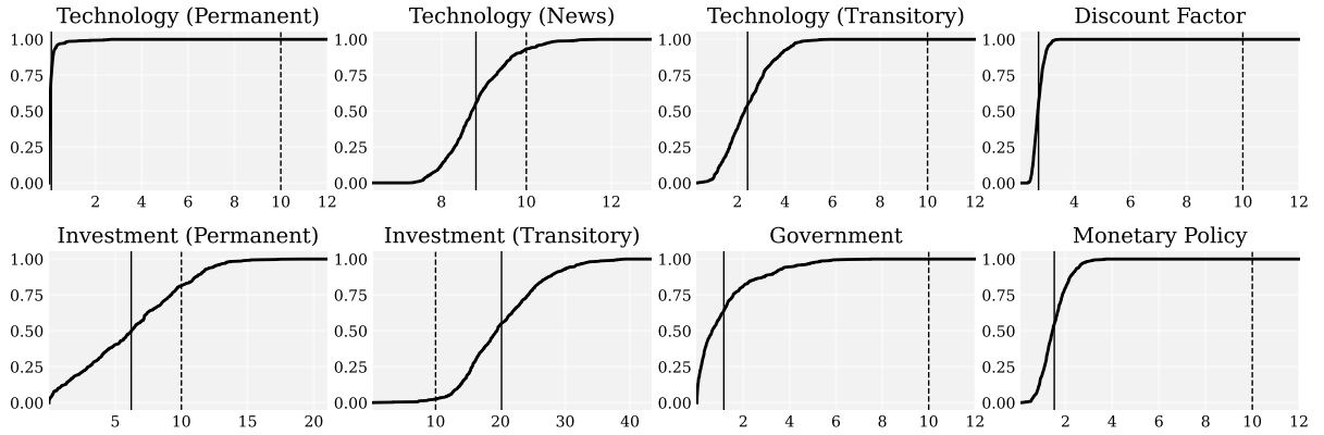
Figure F.1: Weak Instrument Test (No HOB shock model)
