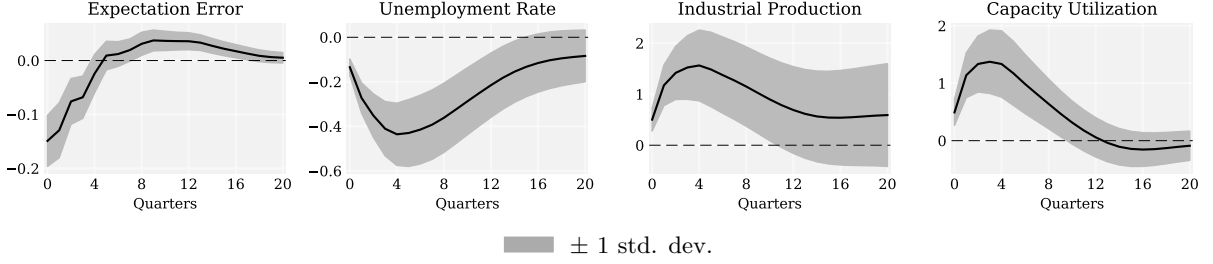
Figure 4: Baseline VAR: Impulse Response to a HOB Shock
