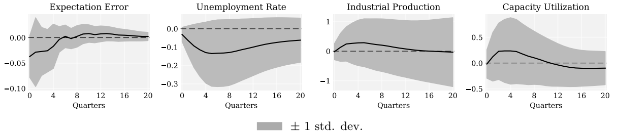
Figure 15: IRF to a (DSGE-) News Shock
