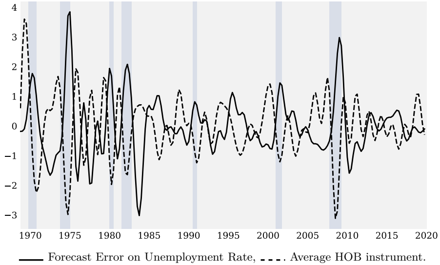
Figure 3: HOB instrument vs Forecast Error on Unemployment Rate
