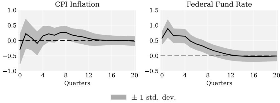
Figure 6: IRF in the Nominal Side
