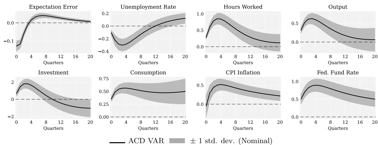
Figure D.1: ACD VAR
