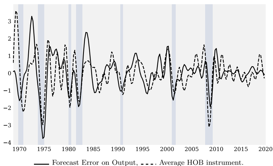
Figure C.1: HOB instrument vs Forecast Error on Output
