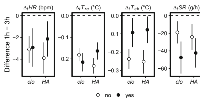
Fig. 3 Least-square means with 95%-confidence intervals estimated by ANCOVA (cf. Table 2) for the main effects of clothing condition ( clo , coded semi-nude = ‘no’, clothed = ‘yes’) and status of heat acclimation ( HA , ‘no’ vs. ‘yes’), respectively, on the difference between 1 h- and 3 h-values ( \Delta_t ) of heart rate ( HR ), rectal ( T_{re} ) and mean skin temperature ( T_{sk} ) as well as sweat rate ( SR )
