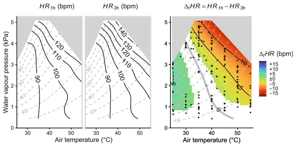
Fig. 4 Contours of heart rates ( HR ) after 1 h (left panel) and averaged over the third hour (3 h) of exposure (mid panel) in relation to air temperature and water vapour pressure as well as their differences ( \Delta_t = \Delta_{1h-3h} , right panel) predicted by GAM for semi-nude, acclimated participants. Dashed reference lines indicate relative humidity (%). Asterisks in the right panel mark the conditions of the 223 exposures. Coloured regions show statistically significant non-zero differences ( P < 0.05 ), while grey areas indicate temperature-humidity combinations not supported by our data
