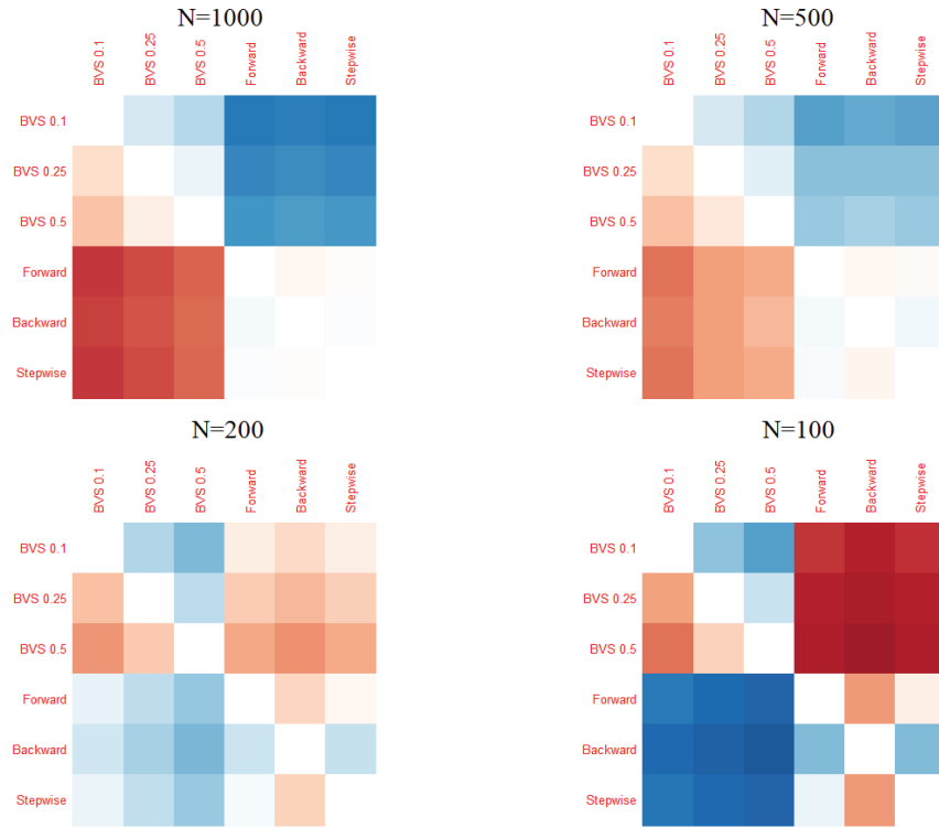
Figure 10: Binary Simulation Results: Heat maps of method-wise average coverage ratio comparisons in binary simulations separated by sample size, where a blue shade represents superiority of the row method in a higher proportion of simulations
