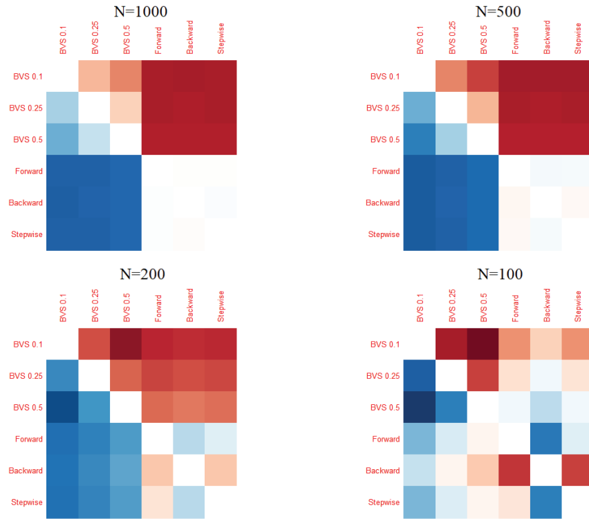
Figure 9: Binary Simulation Results: Heat maps of method-wise average coverage length comparisons in binary simulations separated by sample size, where a blue shade represents superiority of the row method in a higher proportion of simulations
