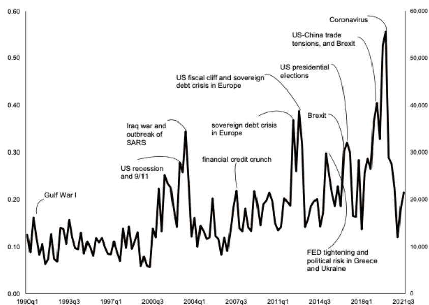
Fig. A1. The World Uncertainty Index 1990–2021.
