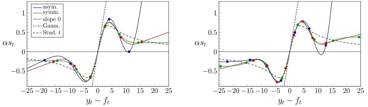
(a) Spline models with k = 6 knots.
