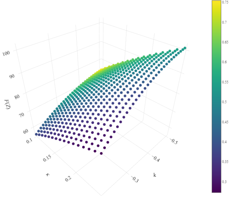
Figure 2: Visualisation of F(\underline{Z}) (Euro/MWh) as a function of k and \kappa , where the colours represent the different related levels of \bar{Z}^* - \underline{Z} (MWh).
