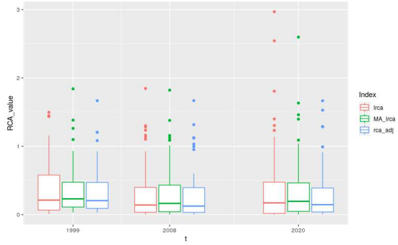
(c) Boxplot
