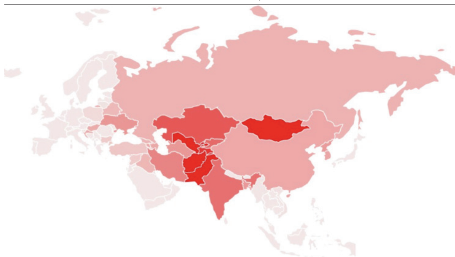
FIGURE 11 Map of M_{\%t}^i
