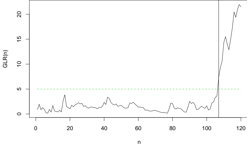
Figure 2: Plot of GLR(n) as a function of n for the data in Fig.1. The stopping time with c_\gamma = 5 is N_G = 107 .
