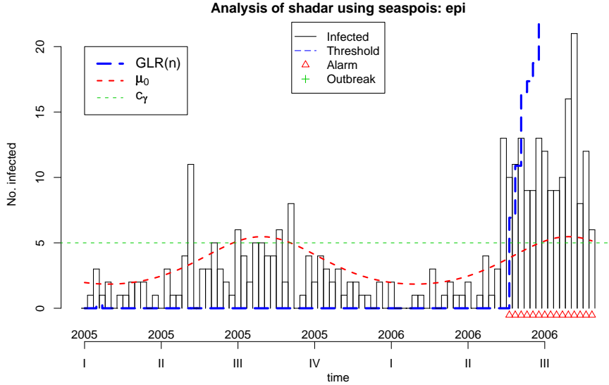
Figure 9: GLR(n) for the epidemic Poisson chart superimposed on the observed salmonella hadar cases of 2005-2006. The triangle shows the first time GLR(n) \geq c_\gamma .
