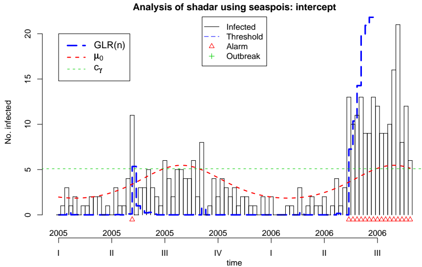
Figure 7: GLR(n) for the salmonella hadar data superimposed on the observed data of 2005-2006. The triangles show all n , where GLR(n) \geq c_\gamma .
