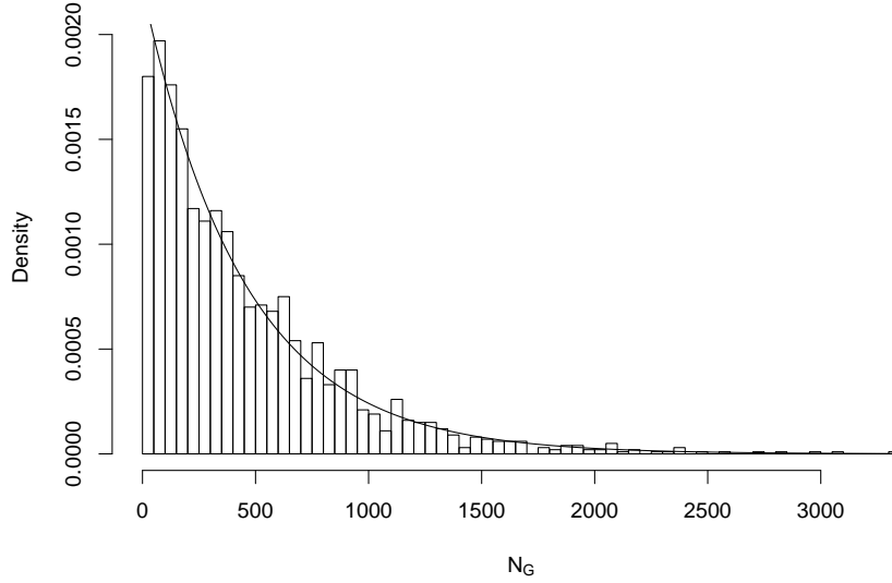
Figure 3: Histogram of the Monte-Carlo RLs N_G^{(t)}, t = 1, \dots, 2000 when c_\gamma = 5 .
