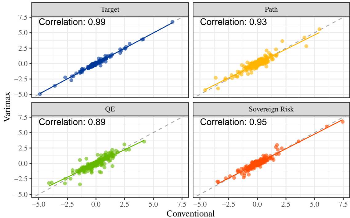
Figure 6: Comparison of the values of the monetary policy factors in each ECB Governing Council meeting estimated with Varimax and with the conventional approach.
