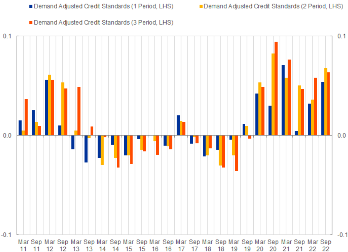
FIGURE 3. Comparison of demand adjusted credit standards with varying backward looking windows
