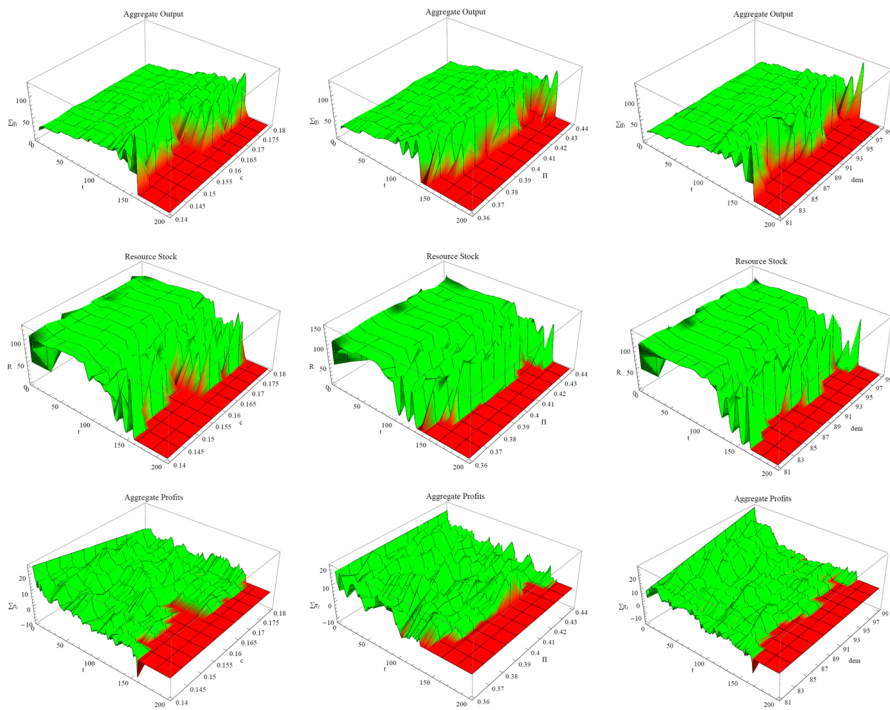
Fig. 5 Sensitivity analysis for \pm 10\% variations of Dem , c , and \Pi
