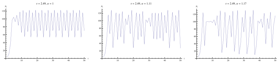
Fig. 1 Effect of a change of an overshooting influence ( \alpha ) from the economic system on the stability of the resource
