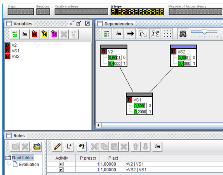
Fig. 4 Example 1iv). Rules (bottom) and marginals in \overline{Q}_- after compression
