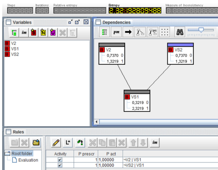
Fig. 5 Example 1iv). Rules (bottom) and sp-values in \overline{Q}_- after compression
