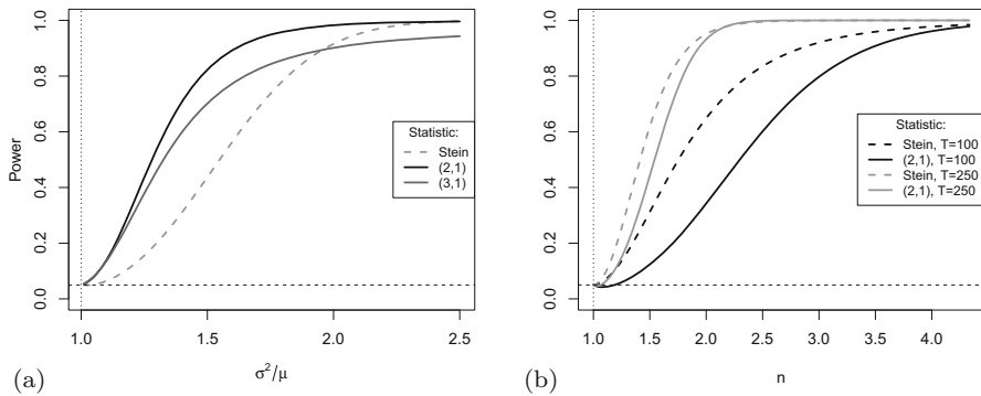
Fig. 2 Asymptotic power curves of Stein tests and some \hat{T}_{(r,s)} -tests (5 %-level) against NB-alternatives with n \neq n_0 and \sigma^2/\mu = 1 + \mu/n , where \mu = 2.5 . a Poi-null with T = 100 using \hat{T}_{\text{exp}}^{\text{Poi}} , and b geometric null ( n_0 = 1 ) with T \in \{100, 250\} using \hat{T}_{\text{exp}}^{\text{NB}}
