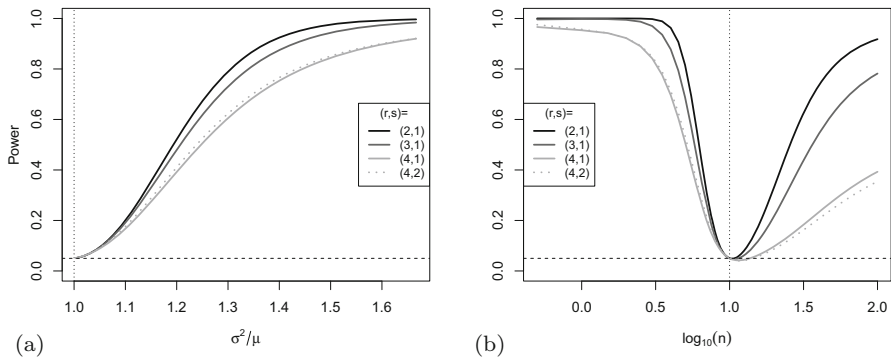
Fig. 1 Asymptotic power curves of \hat{T}_{(r,s)} -tests (5%-level) for null hypotheses a Poi-INAR(1) (so n_0 = \infty ) and b NB-IINAR(1) with n_0 = 10 (see dotted lines). NB-IINAR(1) alternatives with n \neq n_0 and \sigma^2/\mu = 1 + \mu/n , where \mu = 5 , \rho = 0.3 , and T = 250 are kept fixed
