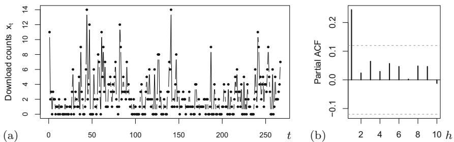
Fig. 3 Time series plot and sample pacf of download counts
