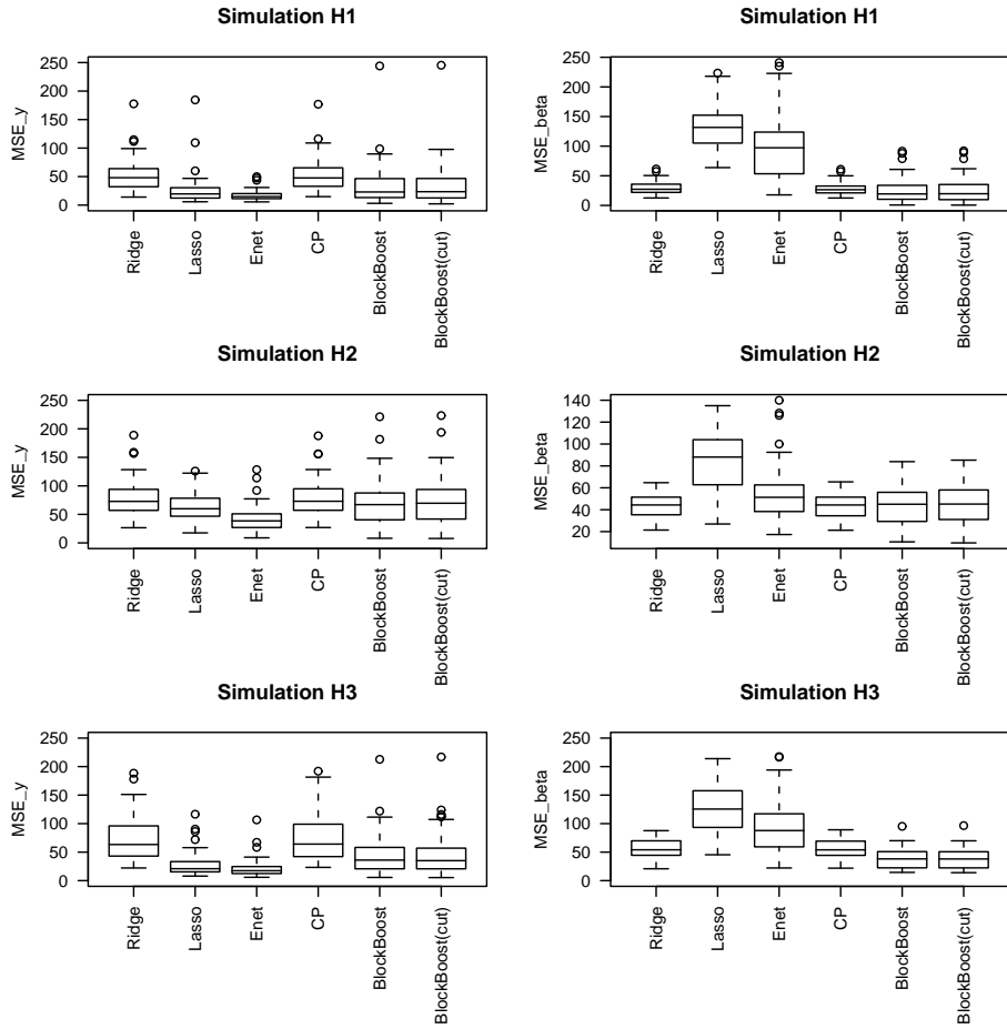
FIGURE 6: Boxplots of test mean-squared errors (left column) and MSE_\beta (right column) for simulations H1 to H3.
