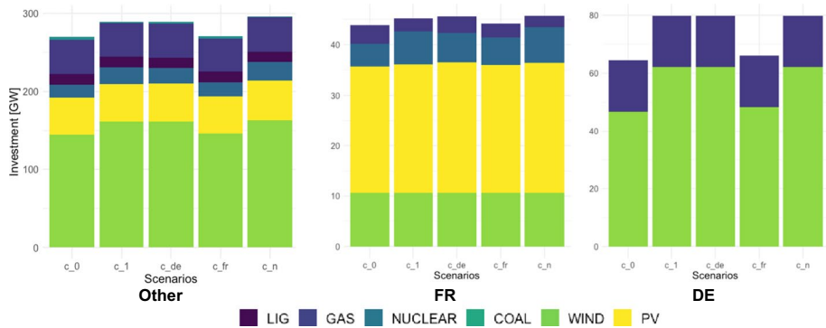
Fig. 7 Investment [MW]
