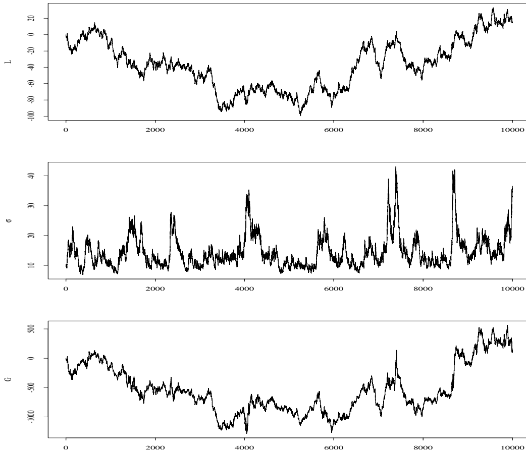
Figure 1: Simulated compound Poisson process (L_t)_{0 \leq t \leq 10000} with rate 1 and standard normally distributed jump sizes ( top ) with corresponding volatility process (\sigma_t) ( middle ) and integrated GARCH process (G_t) ( bottom ). The parameters were: \beta = 1 , \delta = 0.95 and \lambda = 0.045 . The starting value was chosen as \sigma_0 = 10 .
