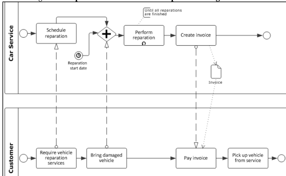
Figure 1. Representation of a business process using BPMN 2.0
