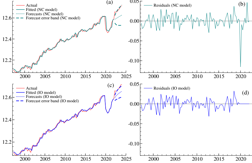
Notes: (a) Dynamic forecasts (NC model), (b) Residuals (NC model), (c) Dynamic forecasts (IO model) and (d) Residuals (IO model). T = 100 , j = 0 , h = 8 , d_t = 0 , \phi = 0.06 and k = 2 . Based on a single replication. The forecast error bands are 95 per cent confidence intervals.
