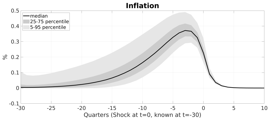
Figure 9: Inflation response
