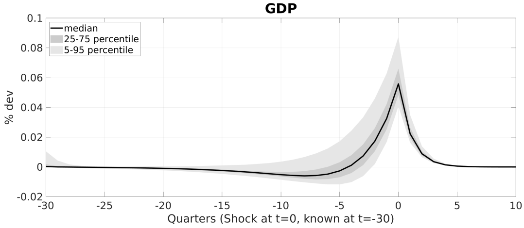
Figure 7: Output response
