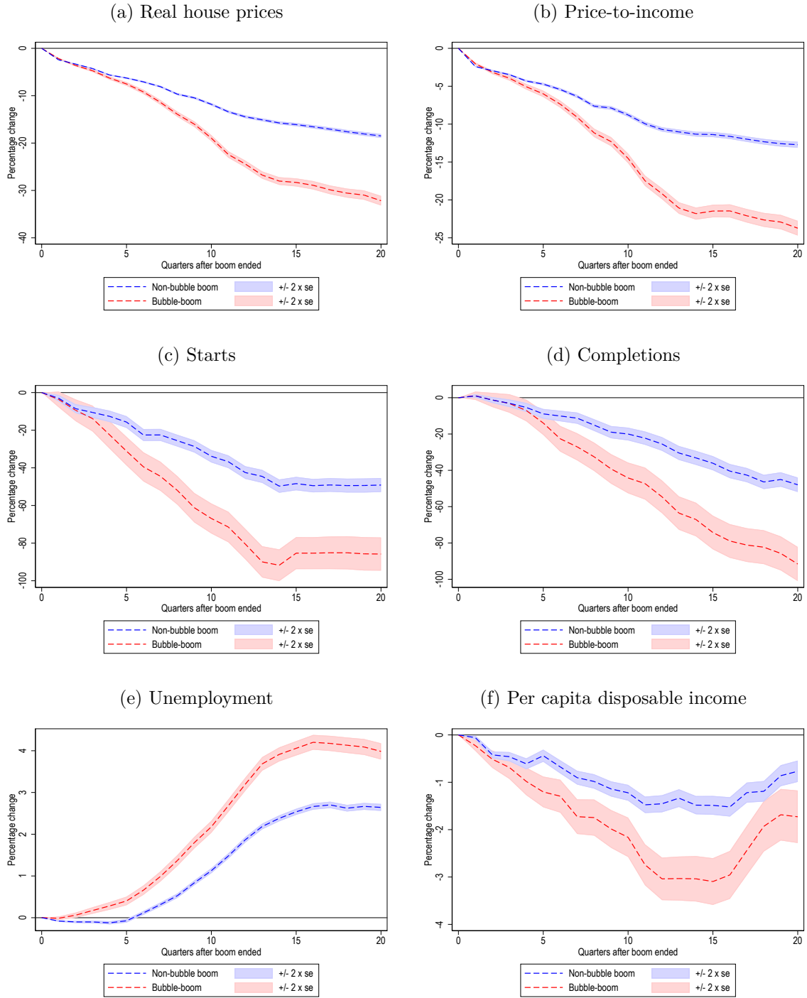
Figure 6: Unconditional paths
