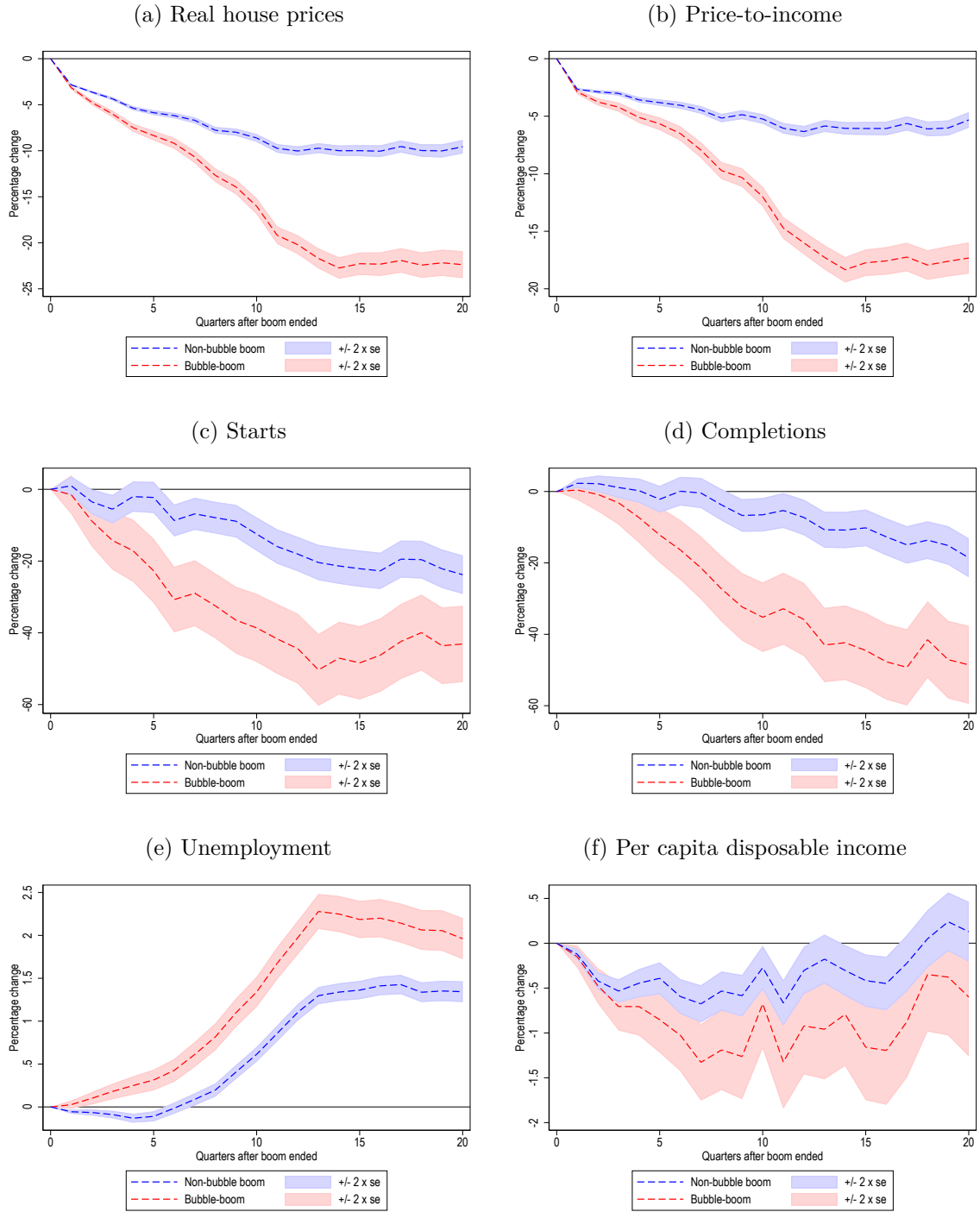
Figure 7: Conditional paths
