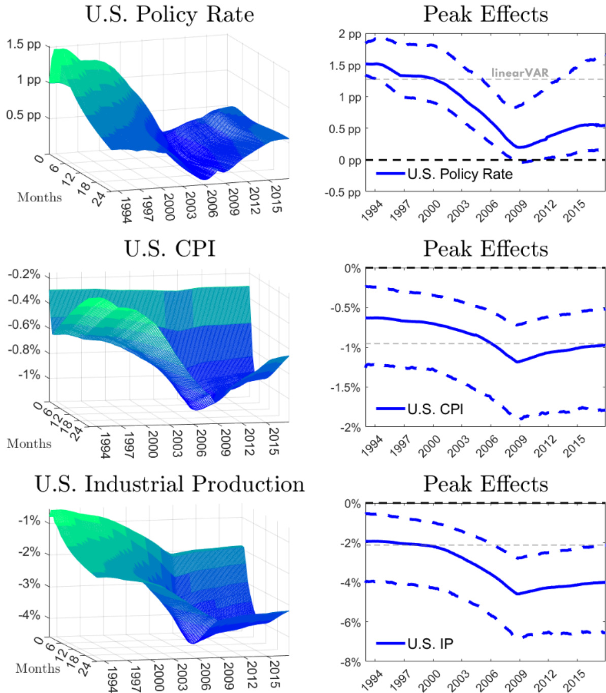
Figure 3: Time-Varying Impulse Responses Functions of Domestic Variables.
