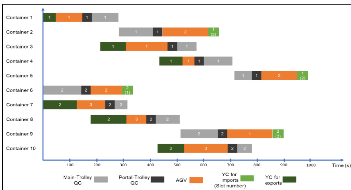
Figure 4. Gantt chart for all equipment used.
