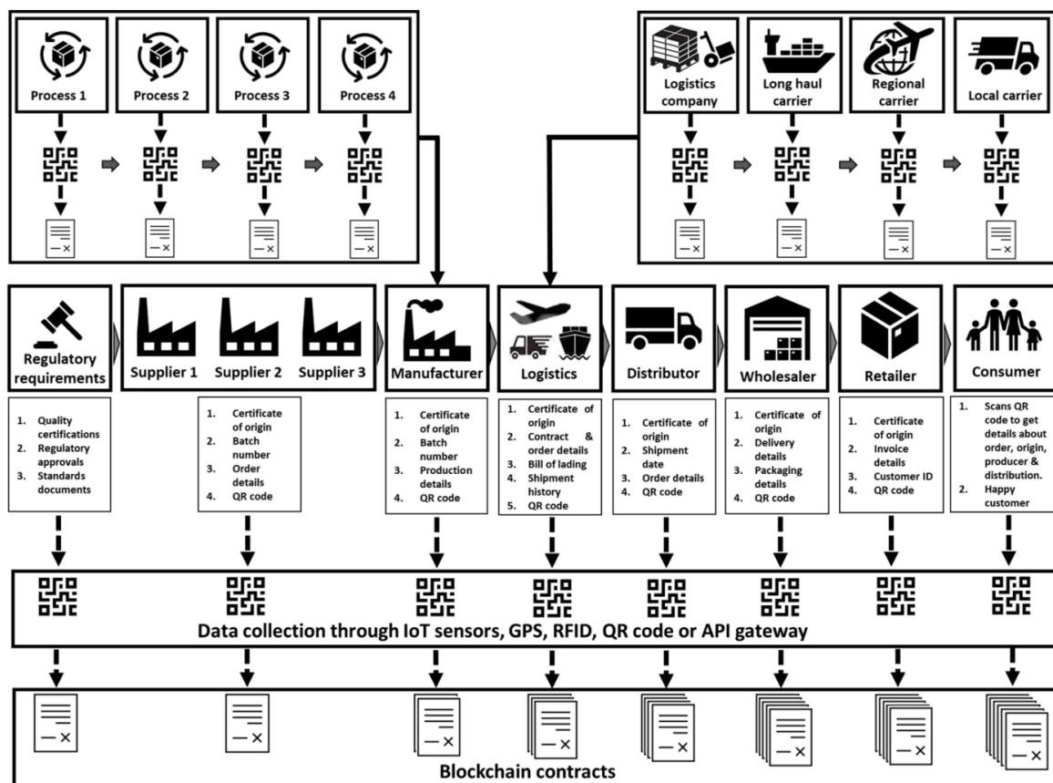
Figure 5. Application of blockchain in supply chain and logistics [9].
