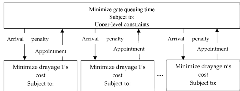
Figure 2. Illustration of interplay between the players.
