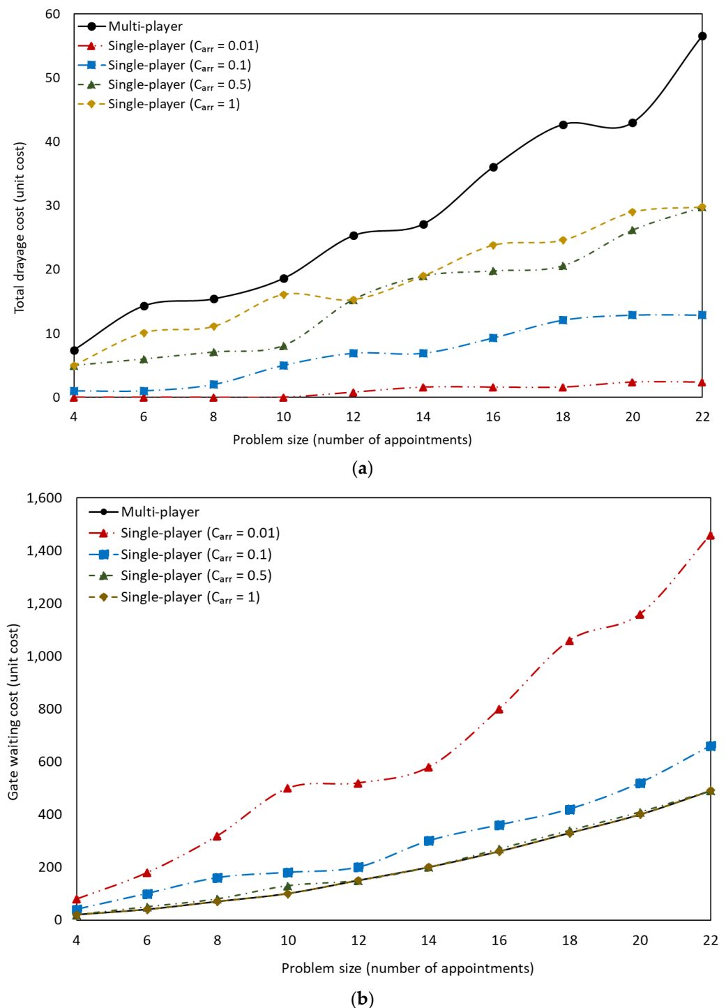
Figure 5. Total drayage cost (a) and post-calculated gate waiting cost (without considering C_{arr} in the last term of Equation (55)), (b) as a function of problem size.
