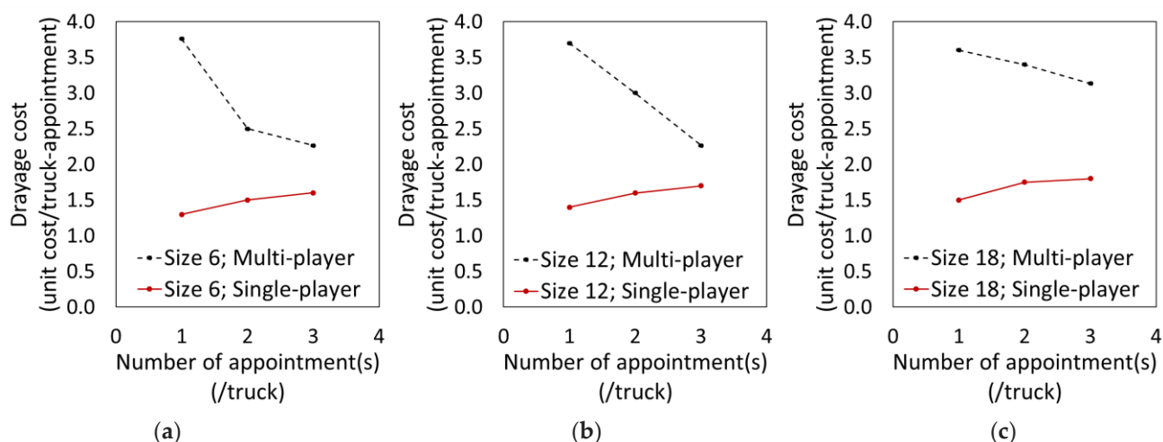
Figure 6. Drayage cost comparison for different problem sizes: (a) 6 appointments, (b) 12 appointments, and (c) 18 appointments.
