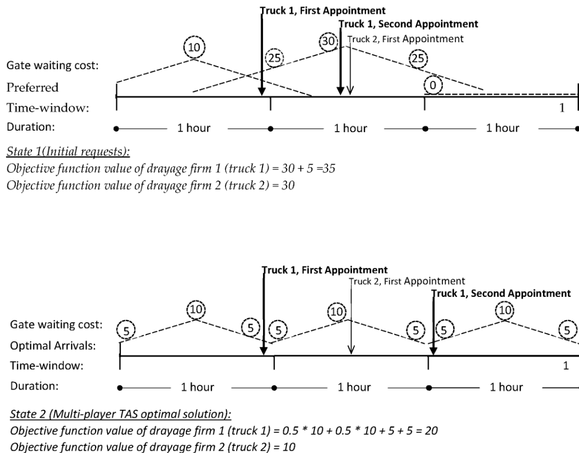
Figure 4. Solution of illustrative example using multi-player TAS.
