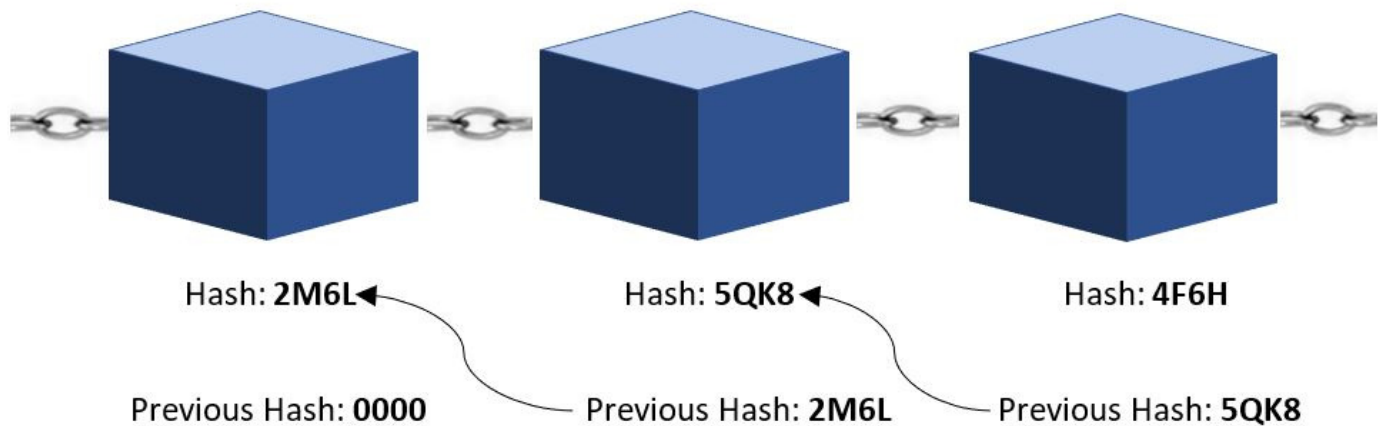
Figure 1. A structure of a blockchain consisting of linked blocks.
