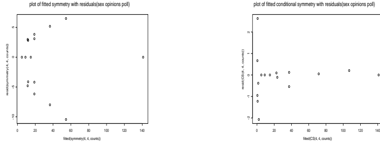
Figure A.1: Fitted symmetry with Residual for sex opinions poll Figure A.2: Fitted conditional symmetry with Residual for sex opinions poll
