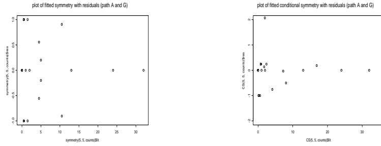
Figure A.3: Fitted symmetry with Residual for path A and G Figure A.4: fitted Conditional Symmetry with residuals for path A and G
